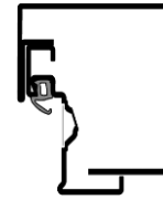
Blockzarge 2-schalig
